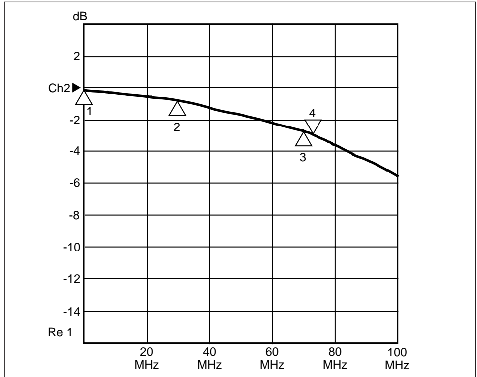
The Model 3000-44 achieves industry-leading performance in excess of 45MHz at -3dB.
